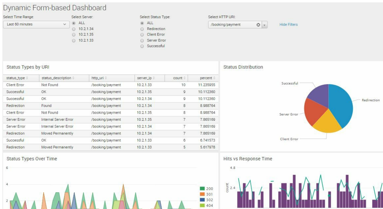
Dynamic dashboard with form input
